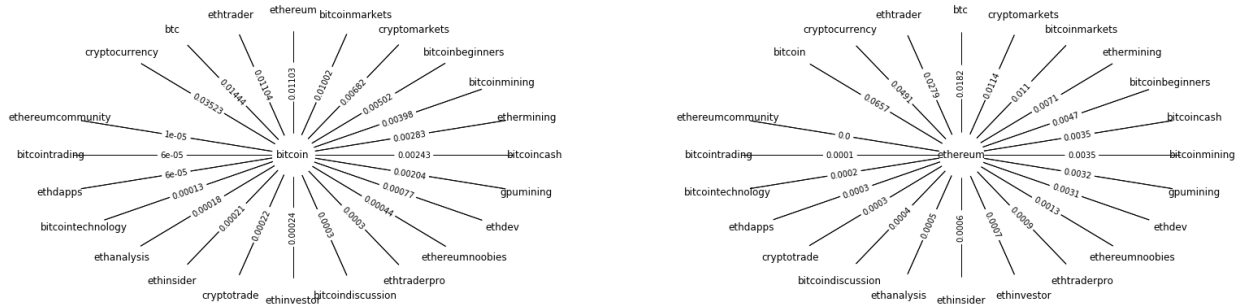
Fig. 2: Personalized PageRank scores relative to 'r/bitcoin' on the left (Fig. 2a) and 'r/ethereum' on the right (Fig. 2b). Figures are ordered in a clockwise direction in a decreasing fashion mirroring the PageRank scores.
