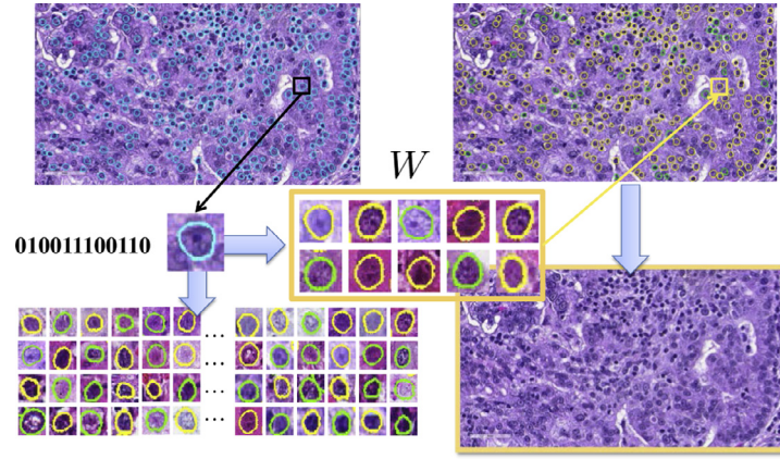
Fig. 3. Workflow of the weighted hashing-based classification. Starting from an unknown image to be categorized, each segmented cell is classified by searching the most similar instances. Their results are combined via the content-aware weighting scheme, predicting the categorization for the whole image.
