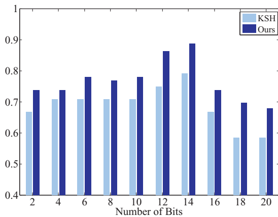
Fig. 6. Classification accuracy of our content-aware hashing and KSH (Liu et al., 2012), using different number of hashing bits (2–20).
