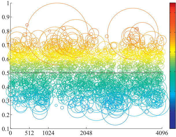
Fig. 2. Illustration of the cell distribution in a hash table. The x -axis means the hash value using 12 bits, ranging from 0 to 4095, and y -axis means the ratio between two types of cells, ranging from 0 to 1. Each circle means a set of cells mapped to the hash value located in the centroid, its size means the number of cells, and the color map visualizes the ratio of two types of cells, same as the y -axis values. (For interpretation of the references to color in this figure legend, the reader is referred to the web version of this article.)
