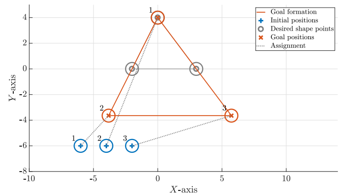
Fig. 3. An example assignment with variable scale formation problem with three robots. The radius R of the robots is 0.5 units. The initial formation of the robots is \mathbf{P} = ((-6, -6), (-4, -6), (-2, -6)) . The desired shape is \mathbf{S} = ((0, 0), (-2, -4), (3, -4)) . The translation parameter \mathbf{d} = (0, 4)^\top is given. The optimal value of \alpha is 1.9111, which corresponds to the lowest cost curve in Fig. 2. The goal formation positions are q_j = \alpha \mathbf{s}_j + \mathbf{d} .
