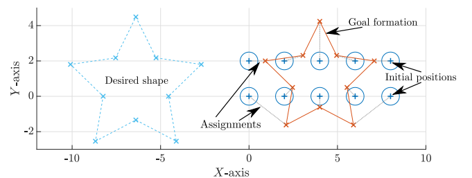
Fig. 1. Illustrative example with ten robots. The circular robots are in two parallel rows in their initial formation. The desired formation shape is a star. The objective is to compute the optimal assignment and the optimal parameters (scale, translation) of the goal formation (indicated by the star with red lines). The assignments are shown by dotted lines. For clarity, the robots are not depicted at their goal positions.
