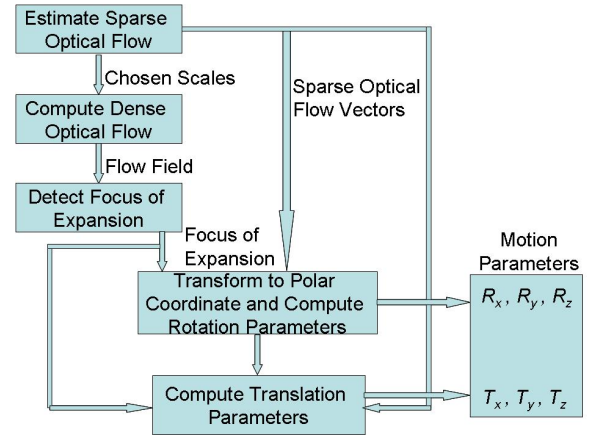
Figure 1. The colonoscopy tracking algorithm.
