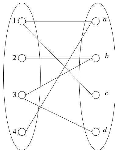
Figure 10.10: The bipartite graph from Fig. 8.1Matches and Perfect Matchesfigure.8.1
