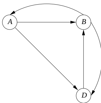
Figure 5.5: The reduced graph with no dead ends
