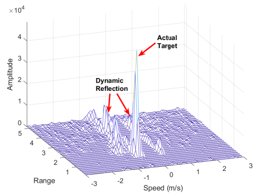
Fig. 5: Highpass-filtered Range-Doppler Map with Dynamic Reflections
